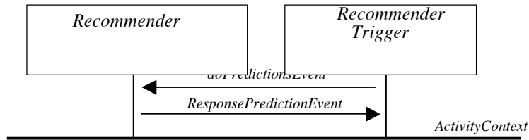
Fig. 2. Communications between recommender and its trigger
