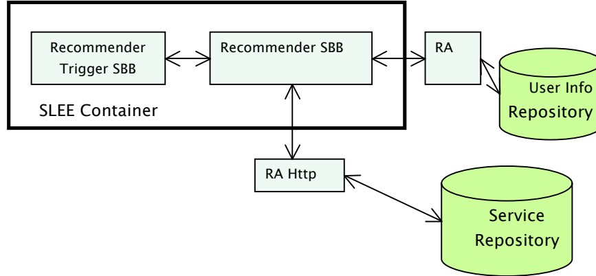
Fig. 1. An architecture of recommender system in telecom domain
